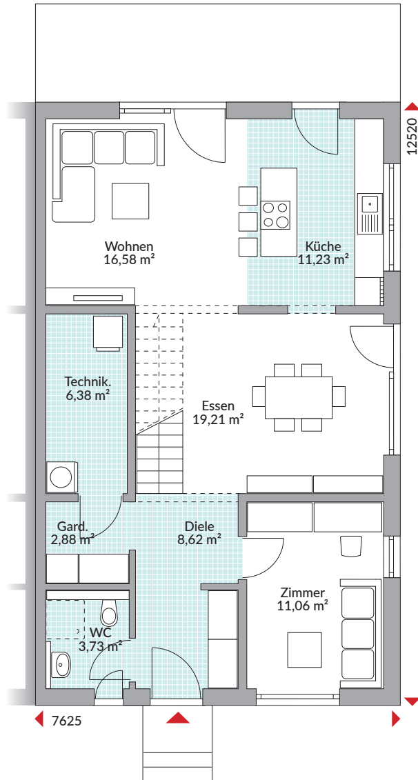
Erdgeschoss 79,69 m 2
